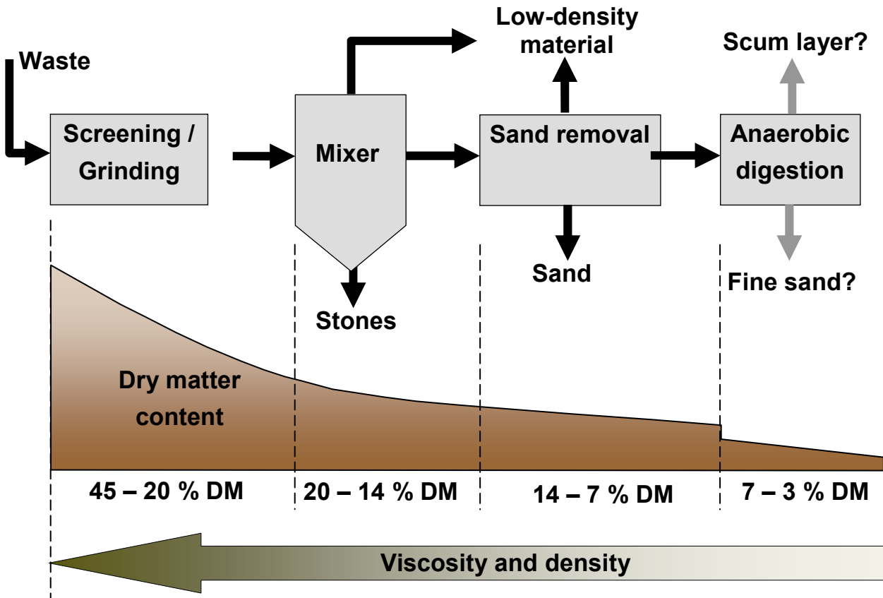
Figure 2 Principle of contraries removal for wet anaerobic digestion
